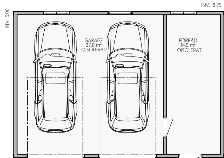
Garage
